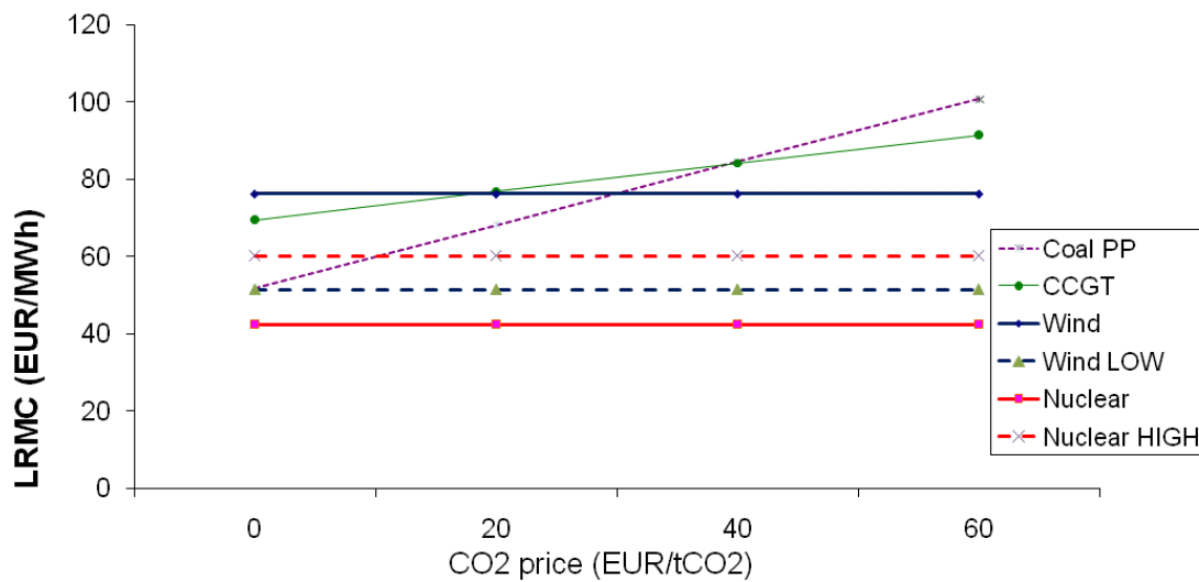
Figure 6. Impacts of emission allowances price on rise of LRMC for different electricity generation technologies, with oil price 84 USD/bbl
