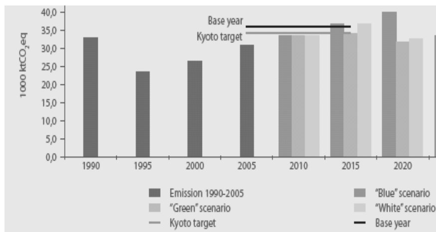
Figure 12. Influence of different scenarios on Croatian Kyoto targets (electricity sector added to total of other sectors) – in year 2015, only Green scenario is meets target, while in 2020 White and Green scenarios are under Croatian Kyoto obligation
