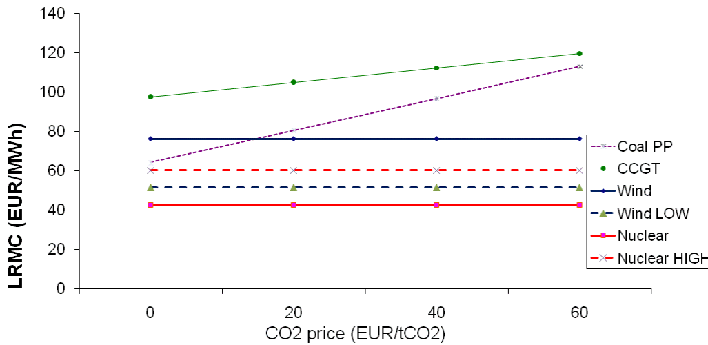
Figure 7. Impacts of emission allowances price on rise of LRM for different electricity generation technologies, with oil price 126 USD/bbl
