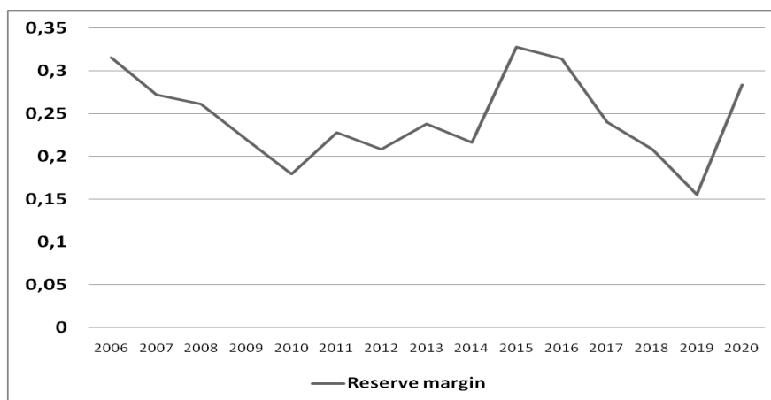
Figure 4. Reserve margin in White scenario fluctuates between 16% and 33% of installed capacity
